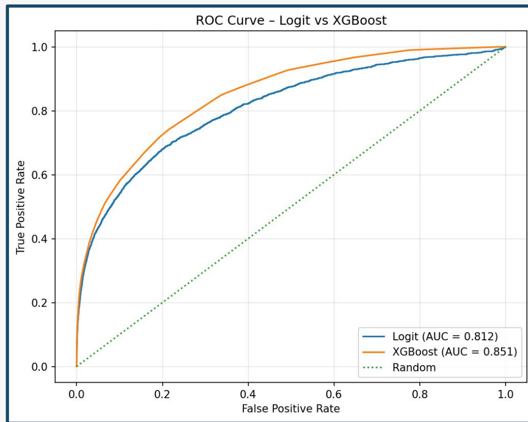
Figure 8 : ROC Curve Between the Baseline Logit Model and XGBoost Model
